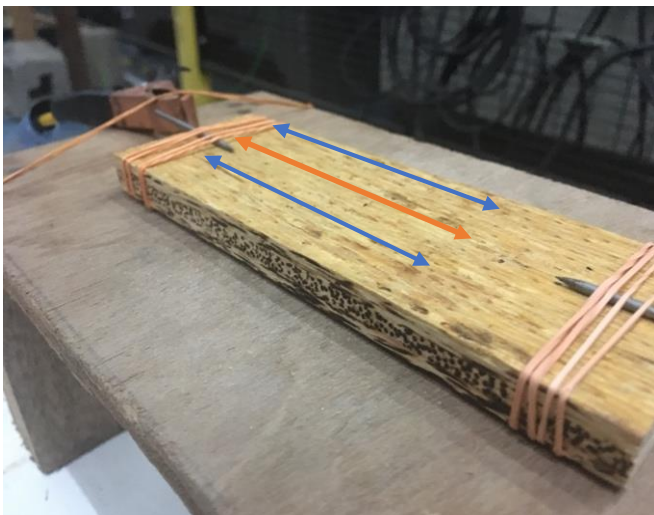
Figure 2: Dry sample with no contamination setup for parallel fiber orientation
