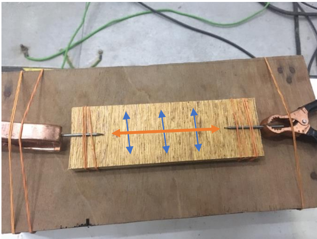
Figure 1: Dry sample with no contamination setup for perpendicular fiber orientation
