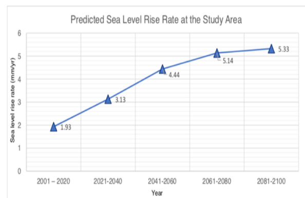
Fig. 4: Mean Sea Level Rise Rate using SRES A1B
