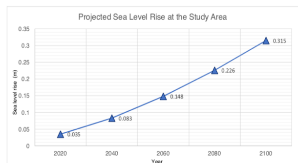
Fig. 5: Mean Sea Level Rise Prediction
