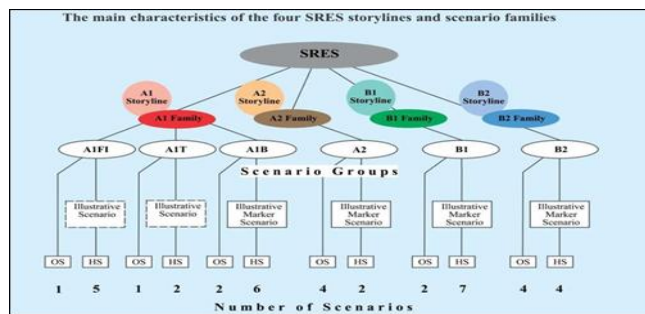
Fig.3: The illustrated storylines and scenarios of AR4 [4]
