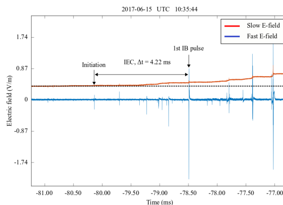
Fig. 2. An Initial Electric Field Change (IEC) (Physic sign convention) and the first Initial Breakdown (IB) pulse for a Negative Cloud-to-Ground (–CG) flash (within reversal distance) captured by wideband fast and slow antenna systems in Malacca at 10:35:44 UTC on June 15th, 2017
