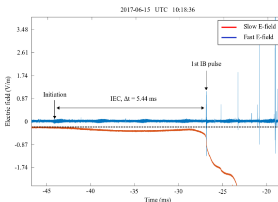
Fig. 3. An IEC (Physic sign convention) preceded the first IB pulse for an Intra Cloud (IC) flash (within reversal distance) captured by wideband fast and slow antenna systems in Malacca at 10:18:36 UTC on June 15th, 2017
