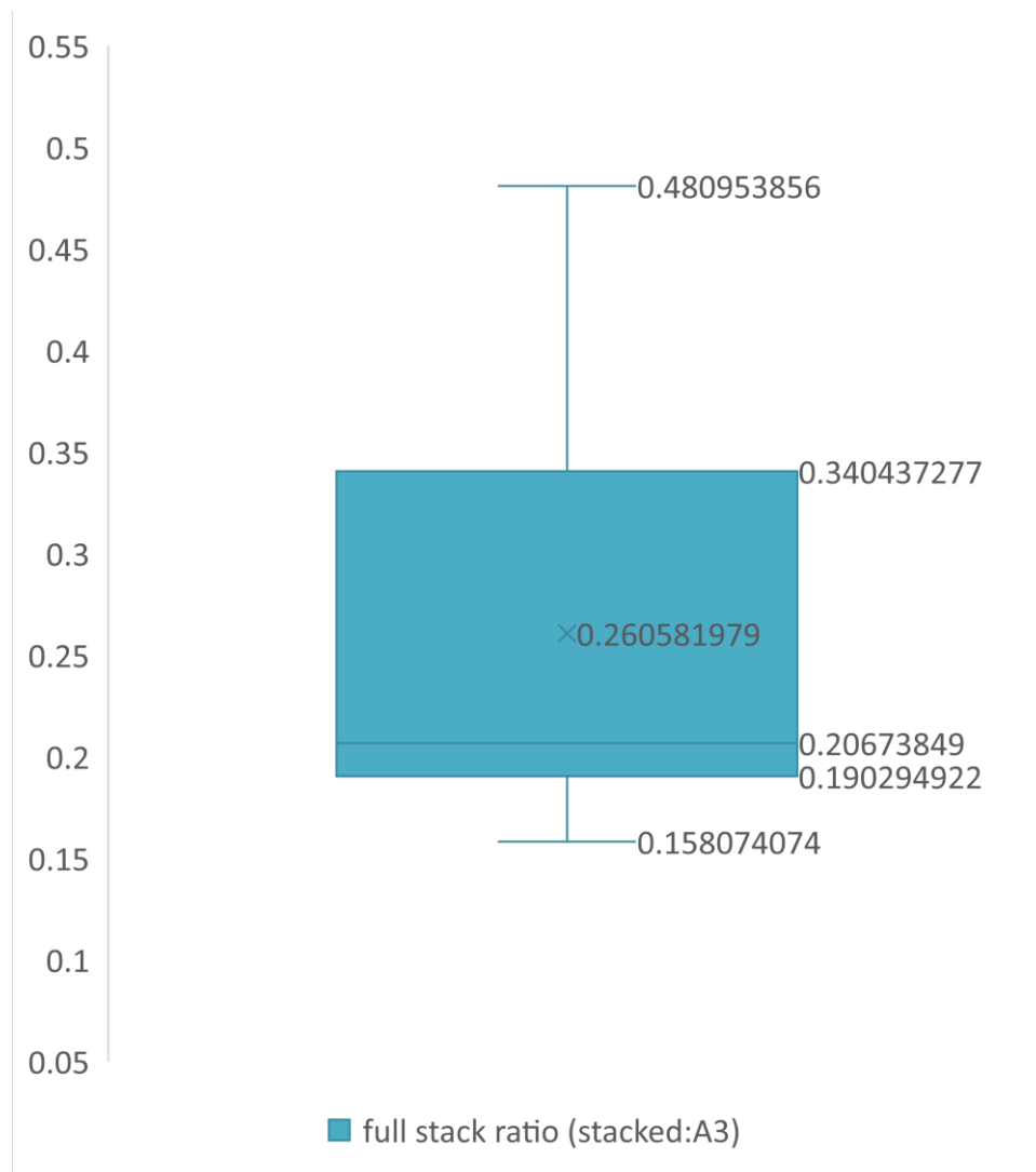
Figure 12: Statistical distribution of the ratio of the 1 st pulse amplitude captured by fully stacked quarter A4 size antenna versus 1 st pulse amplitude of the waveform captured by A3 antenna for each corresponding spark
